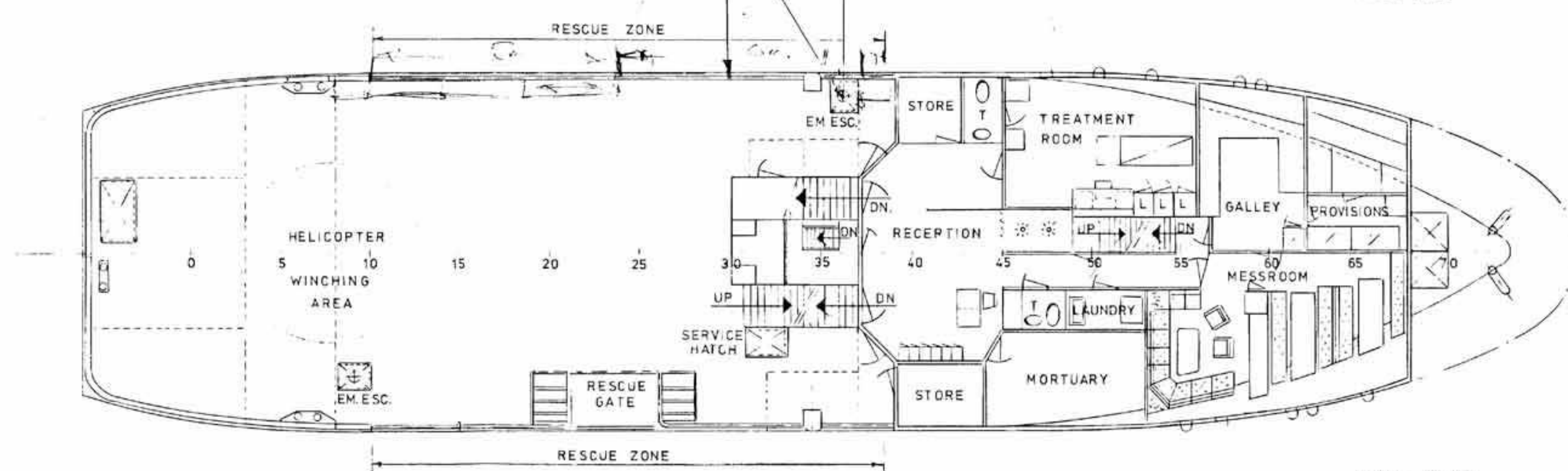
MAIN DECK
