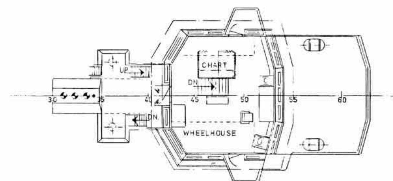
BRIDGE DECK
