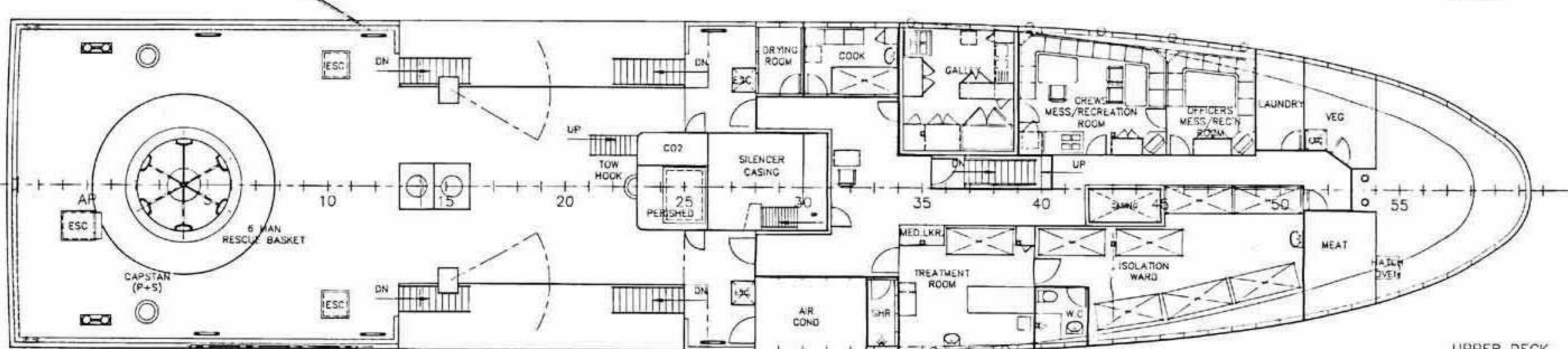
UPPER DECK SURVIVORS 18 BEDS 34 SEATS
